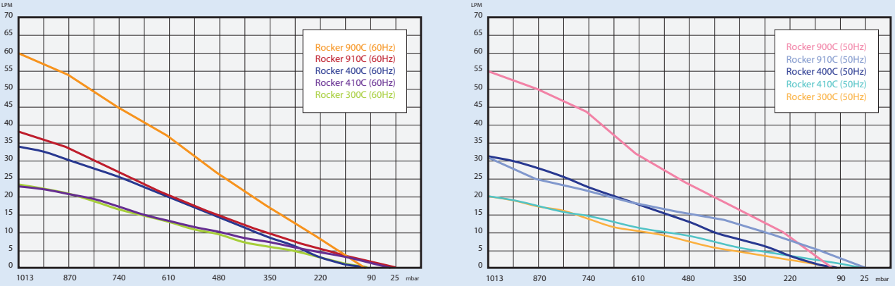
Pumping Speed Graph
